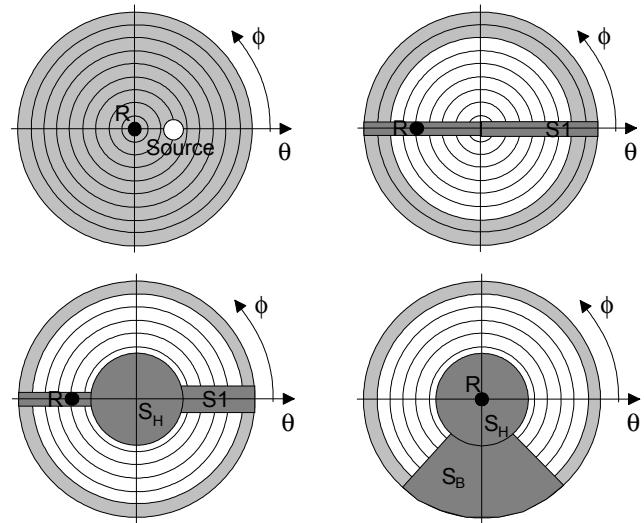
Figure 2: Sketch of the realization of a versatile setup for illumination and detection with a double-layer dome centered around the measuring spot.
